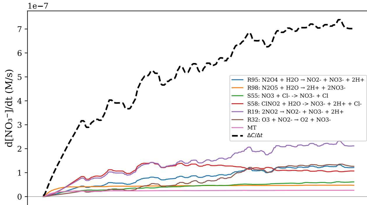
(a) \text{NO}_3^-
